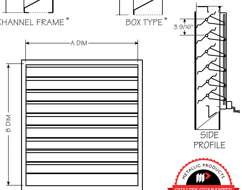
FLAT FLANGE
