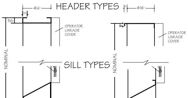
CHANNEL FRAME*
