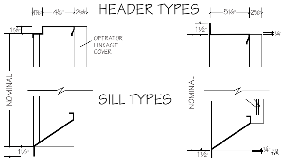
SELF-FLASHING
