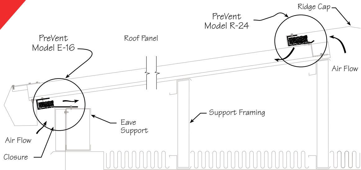
RETRO FIT ROOF APPLICATION Ridge and Eave Vents
