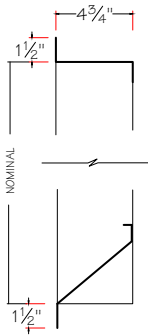
FLAT FLANGE
