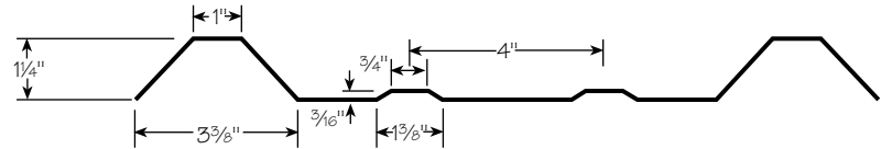
"R" PANEL
