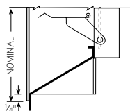
FLAT FLANGE
