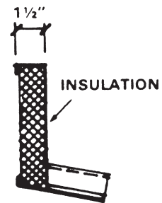
SECTION A-A MP-RC2 INSULATED WHEN SPECIFIED
