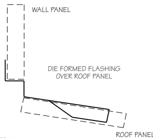
ROOF PANEL
