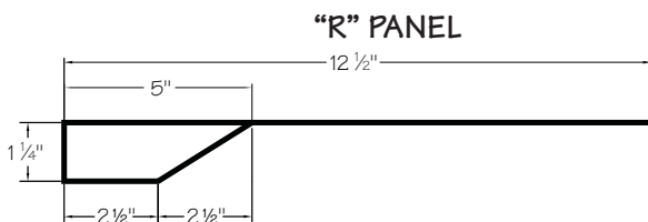
Wall-to-Roof Flashing
