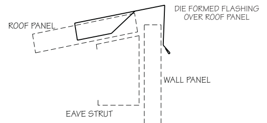
High-Side Eave Flashing
