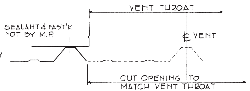
SECTION ALONG RIDGE
