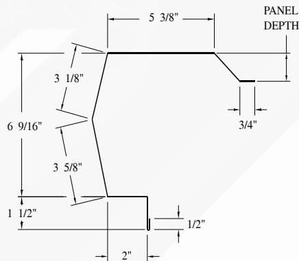
SCULPTURED RAKE TRIM - RT2
