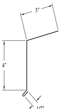
SIMPLE EAVE TRIM - ET5
