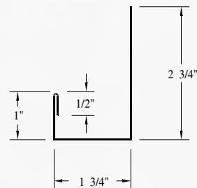
HEAD TRIM - HT19
