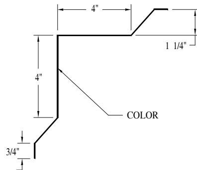
INSIDE CORNER "R" PANEL - CT8
