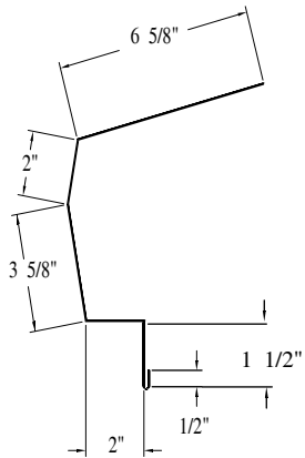
HIGH SIDE EAVE TRIM - ET4
