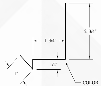
HEAD TRIM - HT18
