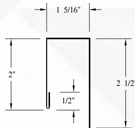
SILL TRIM - ST20
