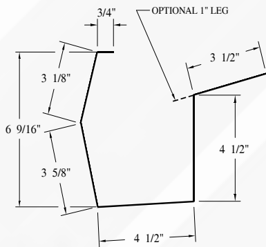
SCULPTURED GUTTER - EG2
