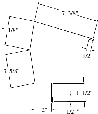
SIMPLE EAVE TRIM - ET5
