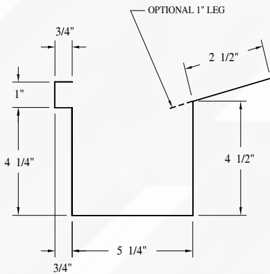
SCULPTURED GUTTER - EG2
