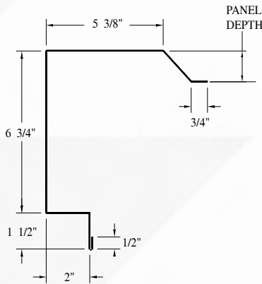
BOX RAKE TRIM - RT1
