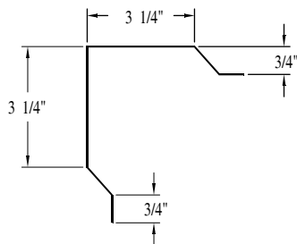
INSIDE CORNER "R" PANEL - CT8
