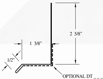
DRIP TRM - DT21
