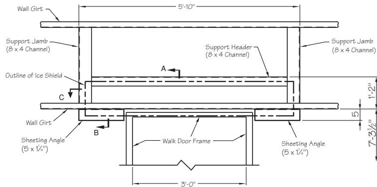
Typical Ice Shield Wall Framing (Single Door)
