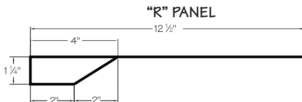
Wall-to-Roof Flashing
