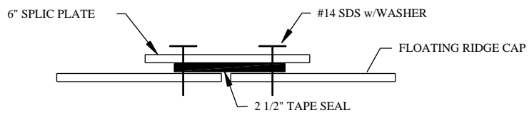
SECTION B
