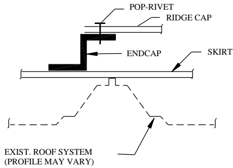
SECTION C
